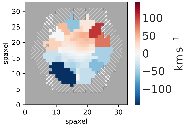
7443-12701 stellar_vel
