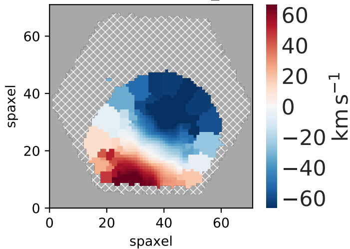
7443-12701 stellar_vel
