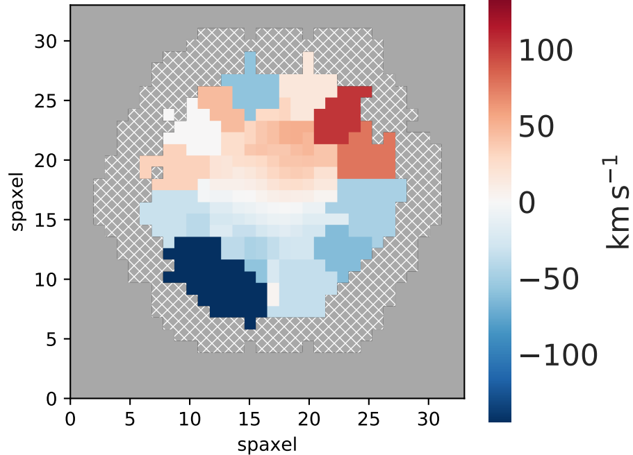
Stellar velocity
