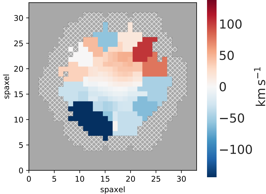
Stellar velocity
