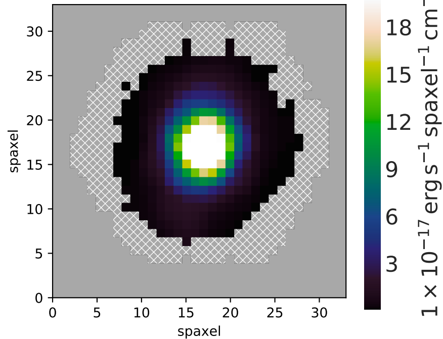
Emission line Gaussian flux: H-alpha 6564
