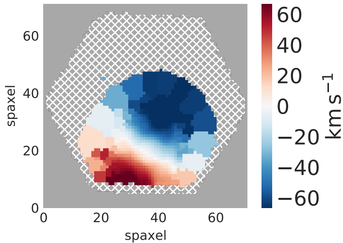
7443-12701 stellar_vel
