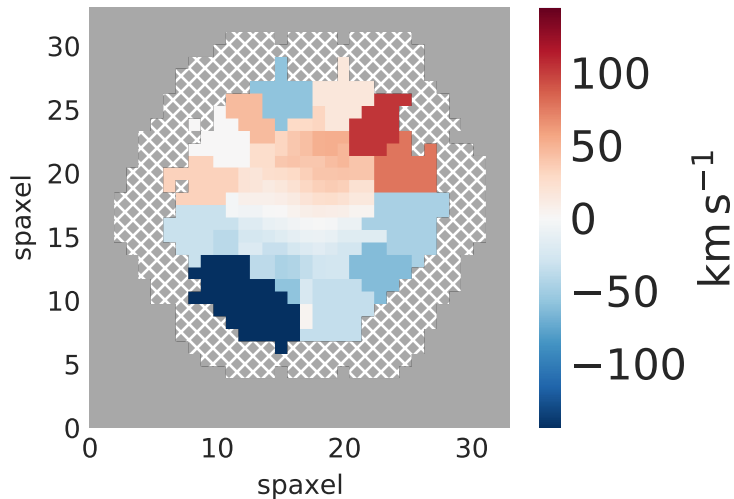
7443-12701 stellar_vel
